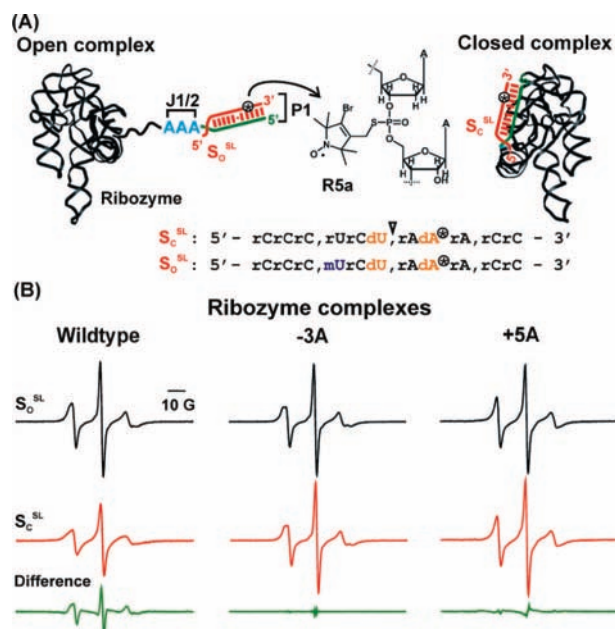
Figure 1. SDSL probing of P1 helix docking. (A) Schematic renditions of the open and closed ribozyme complex. The substrate sequences, the R5a spin label (*), the cleavage site (∇), and the J1/2 junction are marked. (B) EPR spectra of various substrate/ribozyme complexes.
